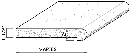
2" BULLNOSE
