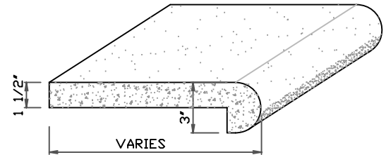
3" BULLNOSE
